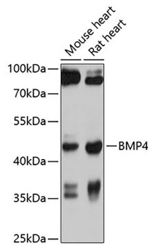
Fig. 1. Western blot analysis of extracts of various cell lines, using BMP4 antibody at 1:1000 dilution. Secondary antibody: HRP-labeled Goat Anti-Rabbit IgG(H+L) (A0208) at 1:1000 dilution. Lysates/proteins: 25µg per lane. Blocking buffer: QuickBlock™ Blocking Buffer (P0231). Detection: BeyoECL Star (P0018A). Exposure time: 1s.
